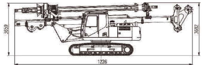
Transportation status(unit:mm)
